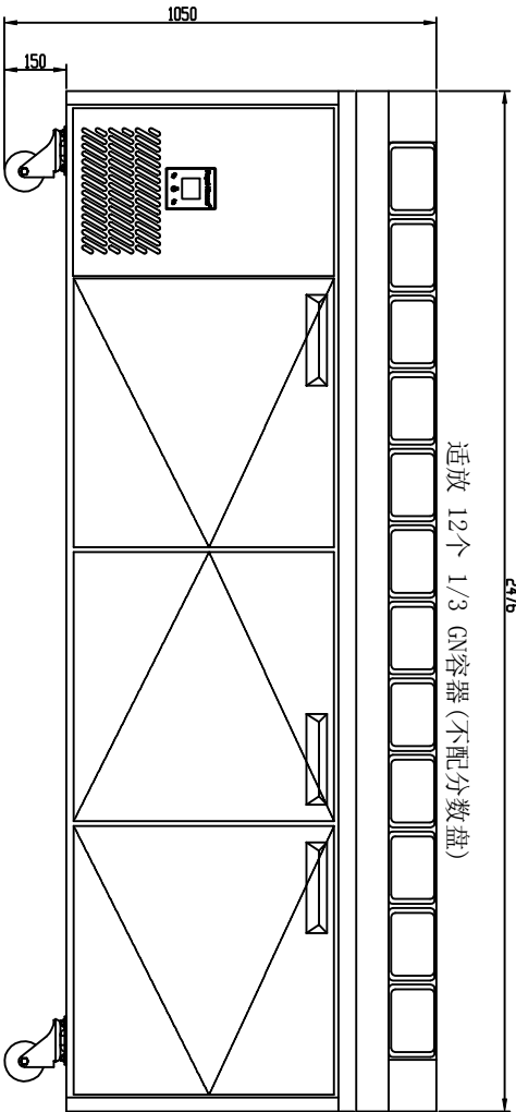
ELEVATION ???
