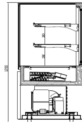
SECTION VIEW
