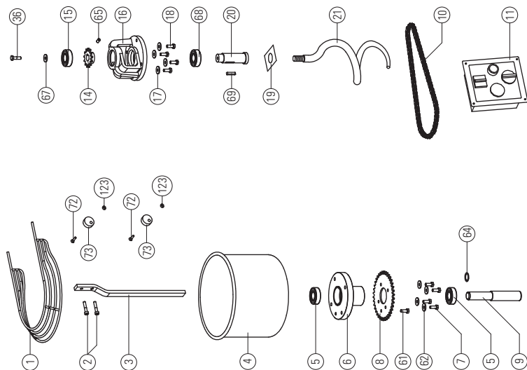
PICT. 19 Spare parts for mixer with fixed top and bowl mod. IM 25-38-44
